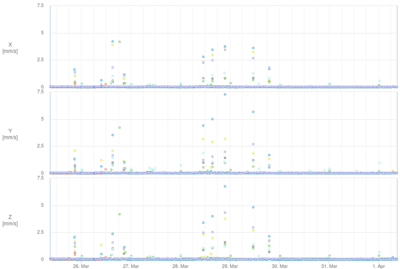
Figure 6. Background recording with 8 MR3000C devices on 1 site
