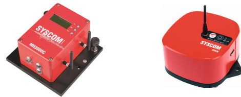
Figure 2. Syscom MR3000C & ROCK vibration monitoring devices
