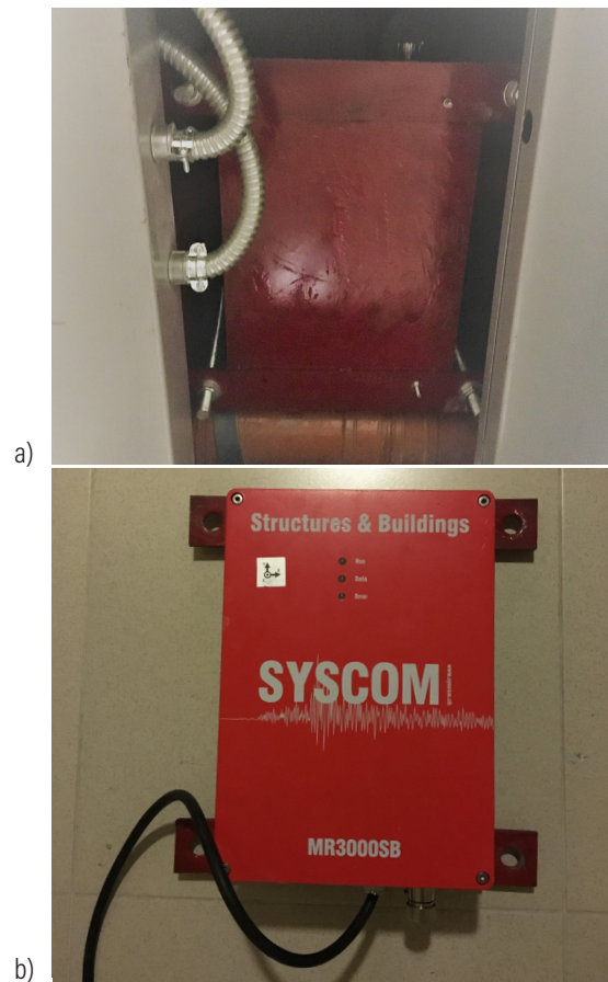
Figure 2. Two MR3000SB used in the project: a) device installed in the ceiling, at the middle floor; b) device ready to be installed in the ceiling, at top floor.
